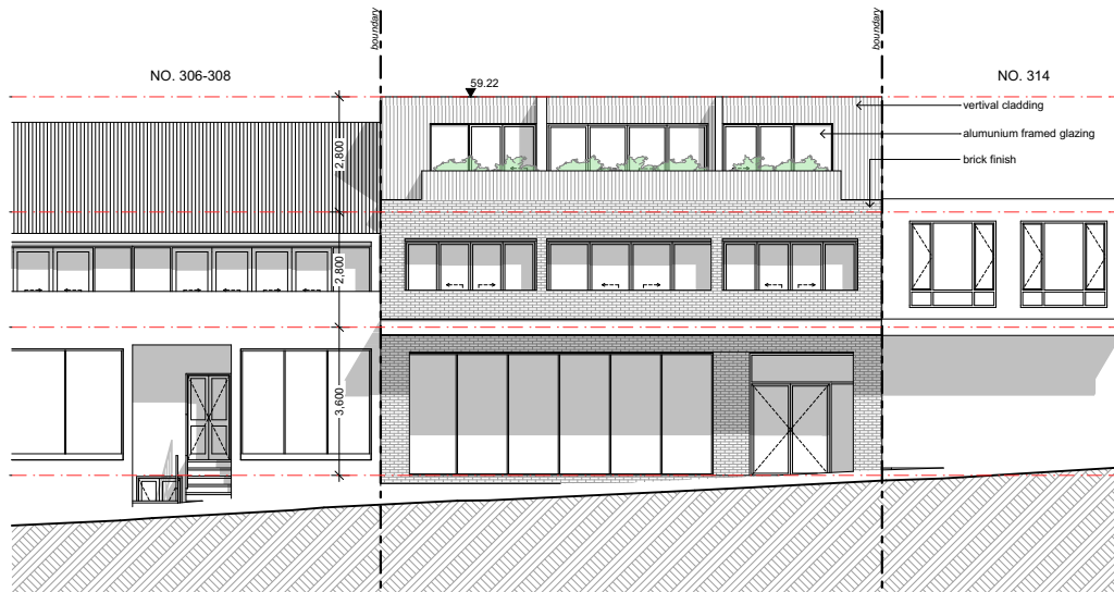
West Elevation (King Georges Road) SCALE 1:200
